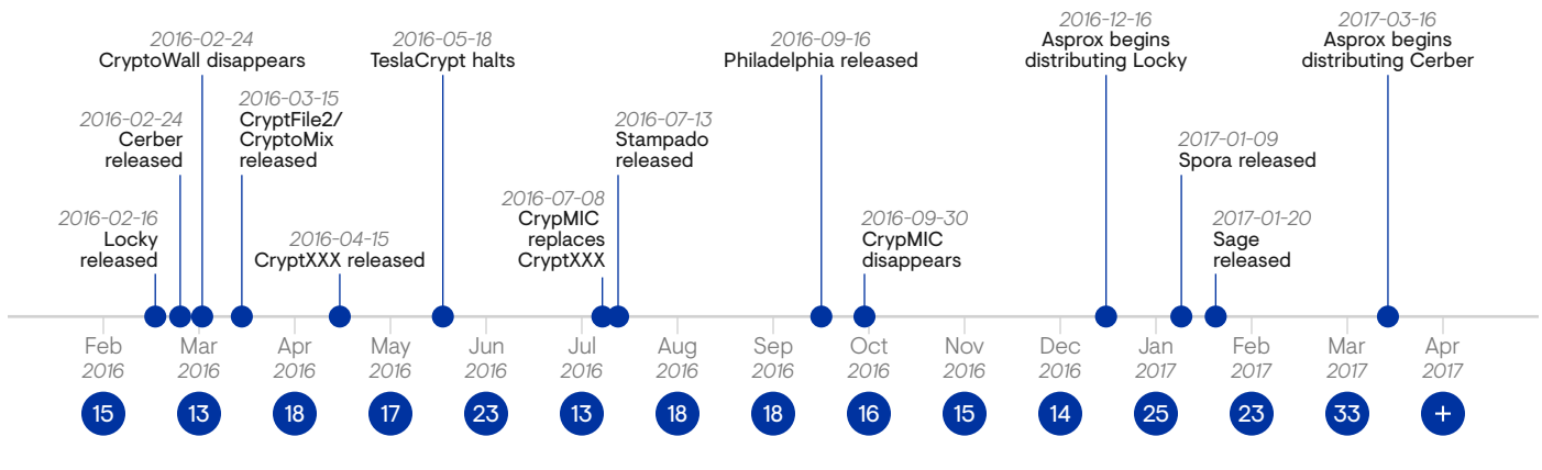
FIGURE 3: Ransomware timeline
