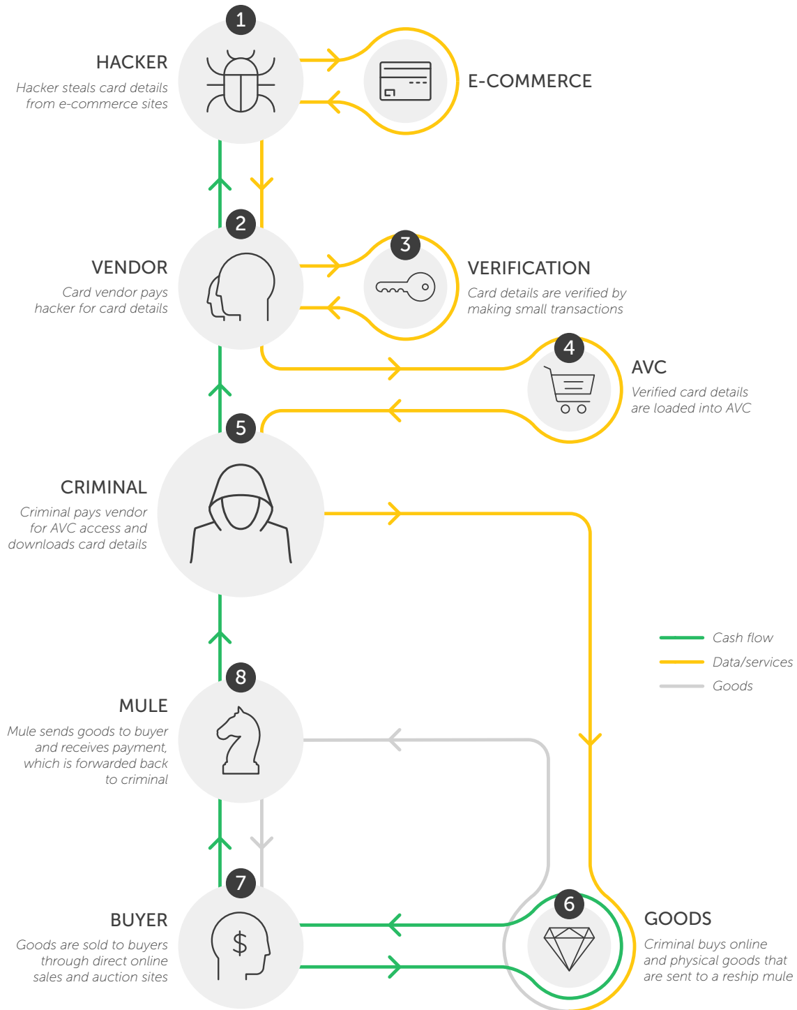
DIAGRAM 3: (Source: Secureworks)
